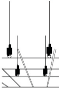
FALSE CEILING SUSPENSION
